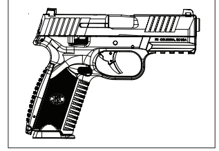
Assembled pistol.
