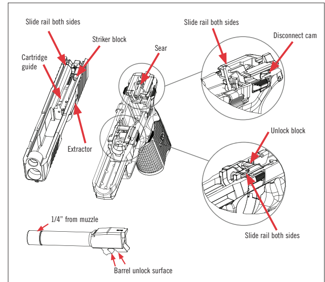
Lubrication Points.
