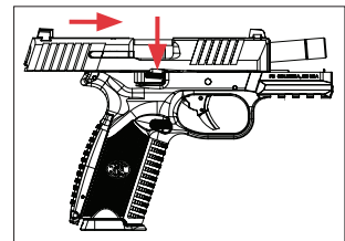
Release slide.
