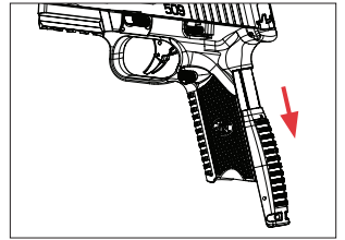
Backstrap removal.
